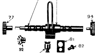
ENLARGED LEVEL WIND PARTS
