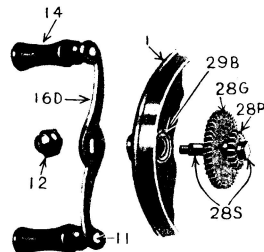
CRANK & GEAR PARTS FOR GEAR STEM BEARING STYLE L.W. REEL LIKE 1905
