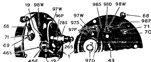
1944 SERVICE THROWOUT PARTS FOR NON-REVERSING CRANK
