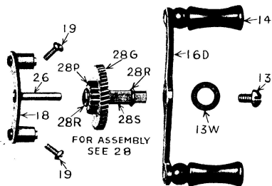
CRANK, GEAR & BRIDGE PARTS FOR 1956 TAKE DOWN STYLE DRIVE GEAR
