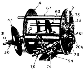
LEVEL WIND PARTS FOR INSIDE TAKE DOWN STYLE
